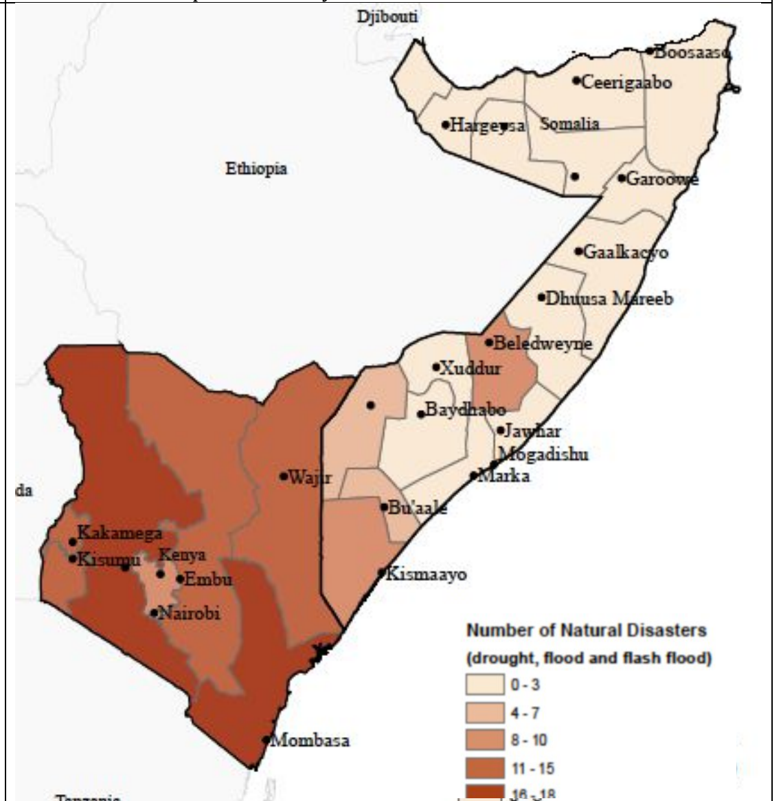
Climate hazards exposure of Kenya
